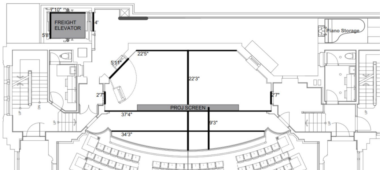
Stage plan with dimensions
